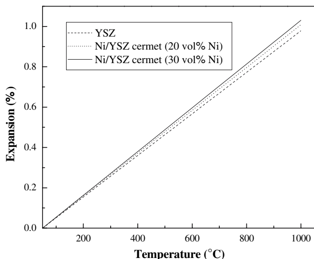
Fig. 6 Thermal expansion of Ni/YSZ cermet and YSZ in inert atmosphere
