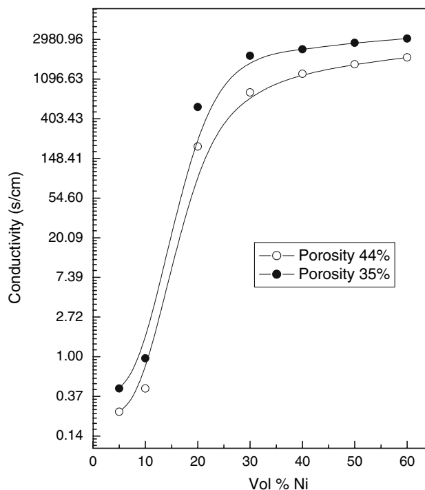
Fig. 10 Electrical conductivity of Ni/YSZ Cermet at 1,000 °C as a function of nickel content and porosity
