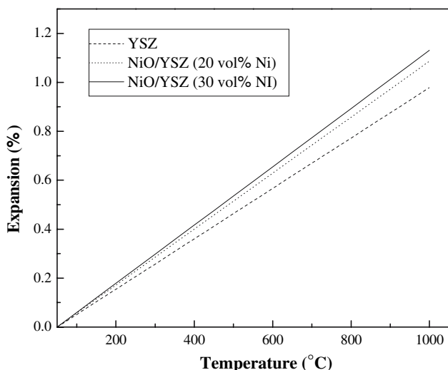
Fig. 4 Thermal expansion of NiO/YSZ composite and YSZ in air
