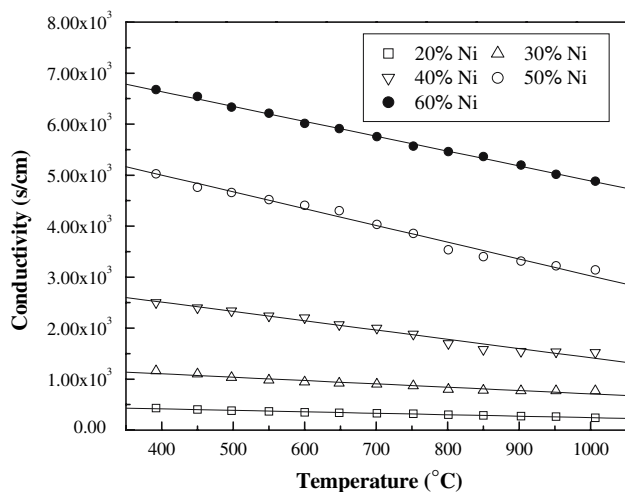
Fig. 9 Temperature dependent conductivity of Ni/YSZ cermet containing 20–60 vol% nickel
