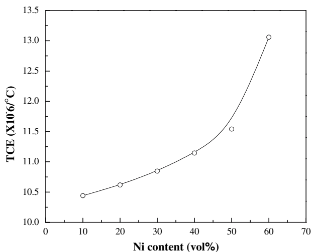
Fig. 7 TECs of the Ni/YSZ cermets from 50 to 1,000 °C in Ar atmosphere. The points are experimental results and the solid line calculated from Kerner's model
