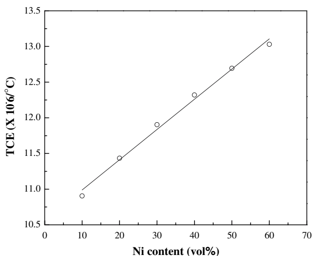
Fig. 5 TECs of NiO/YSZ composite from 50 to 1,000 °C in air. The points are experimental results and the solid line calculated from Kerner’s model
