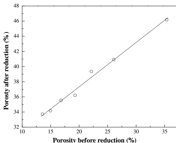
Fig. 1 Relationship between porosities of air-fired and hydrogen reduced Ni/YSZ cermet
