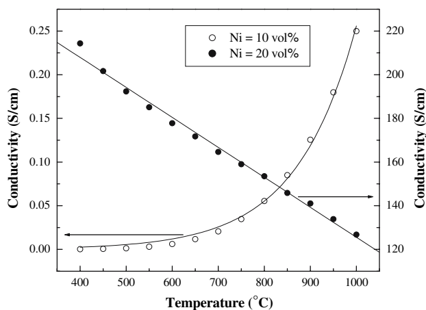
Fig. 8 Conductivity of Ni/YSZ cermet as a function of temperature
