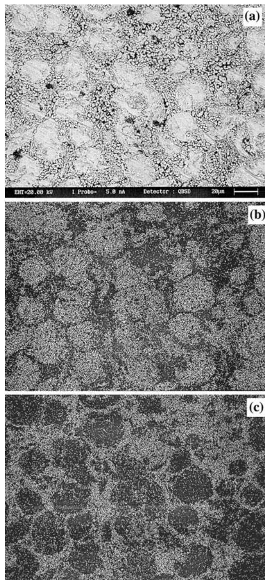
Fig. 3 Back scattered image (a), Zr-distribution (b) and Ni-distribution (c) in 40 vol% Ni/YSZ cermet prepared by electroless coating technique
